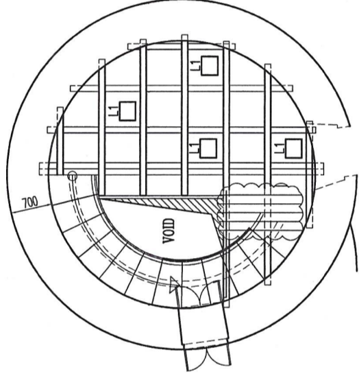
PLAN SHOWING MEZZANINE FLOOR
